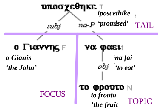
Figure 2: A Greek dependency tree with a communicative partition
