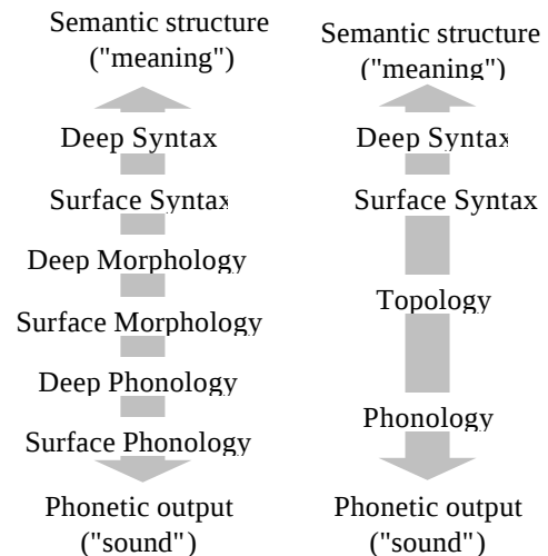
Figure 1: The levels of representation in classical Meaning-Text Theory (left) and our adaptation (right)
