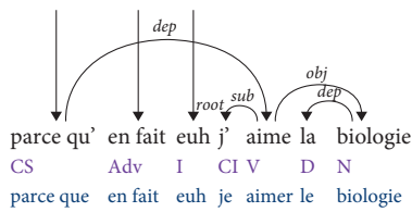
Figure 10. Arborator display of Table 7
