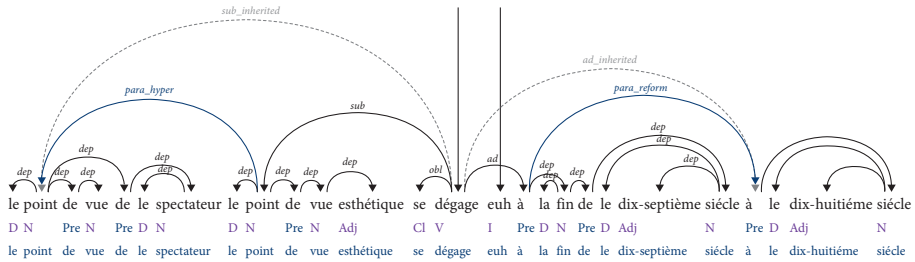
Figure 4. Resulting dependency structure of example (4)
