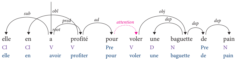
Figure 6. The resulting Rhapsodie dependency structure
