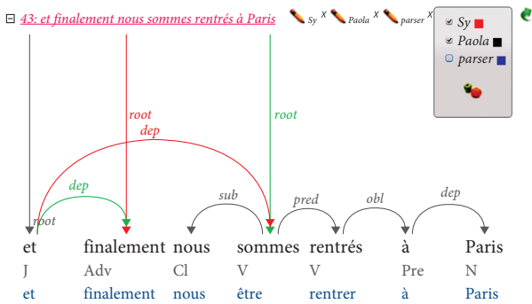
Figure 9. The comparison mode shows the differences between annotations (identical annotations in gray)
