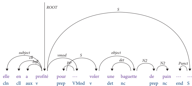
Figure 5. The FRMG dependency structure
