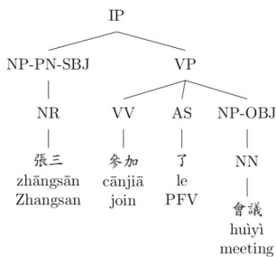
(1a) Constituent tree (CTB)
