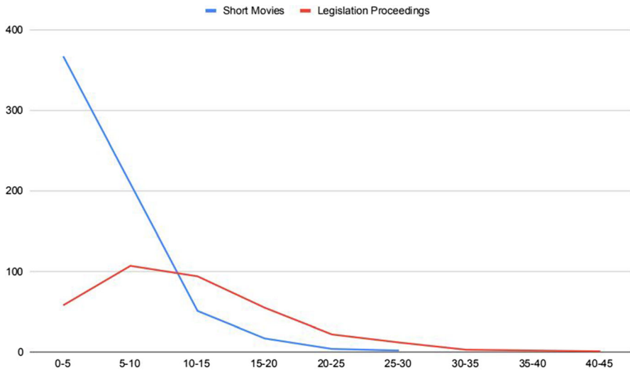
Fig. 1 Distribution of sentences length in the UD Chinese HK treebank
