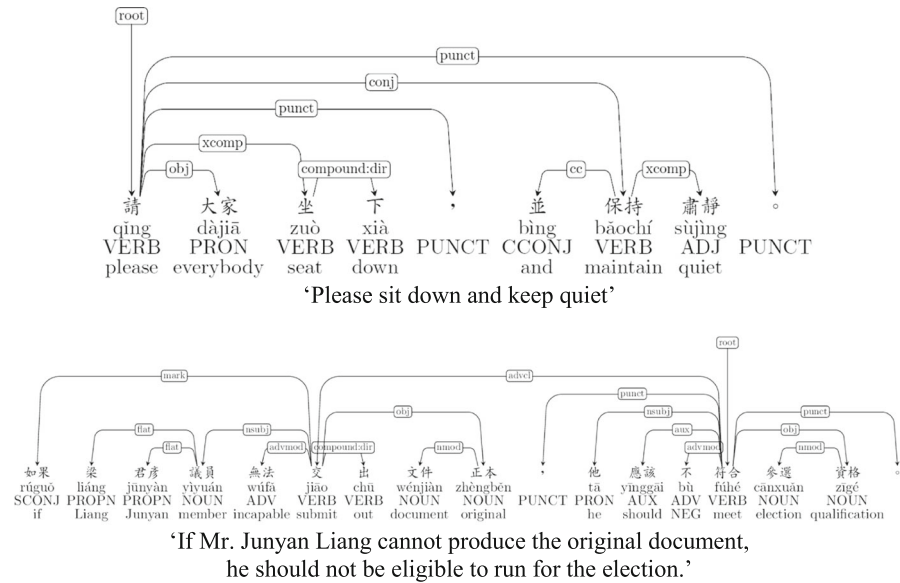
Fig. 3 The marking of the structural relation between two clauses
