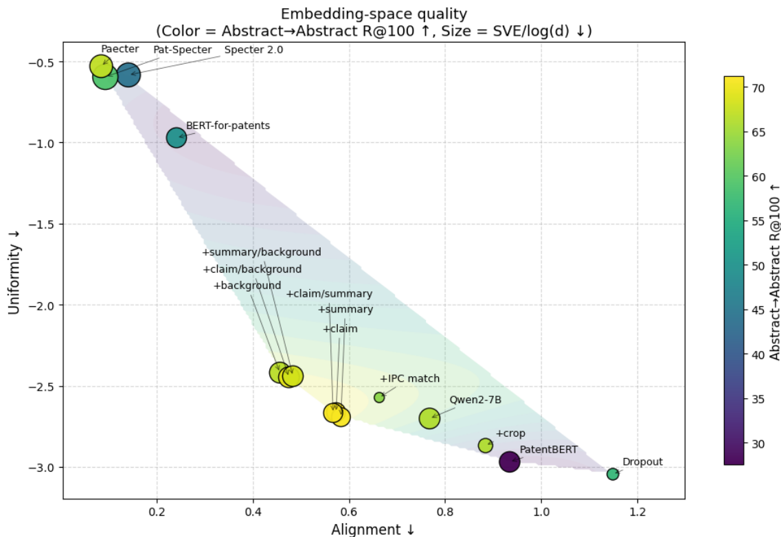
Figure 3: Embedding-space diagnostics. Each point shows alignment (x-axis) and uniformity (y-axis), dot size encodes normalized SVE, and color encodes prior-art retrieval performance (R@100, Abstract→Abstract). Contours indicate an RBF-smoothed performance field within the convex hull of observed points.
