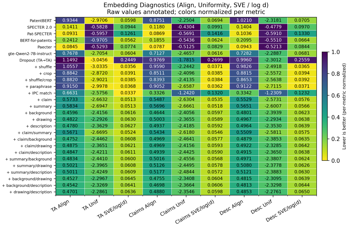
Figure 5: Embedding Space Diagnostics across three patent sections: Title+Abstract (TA), Claims, and Description. We report Alignment ↓, Uniformity ↓, and Singular-Value Entropy (SVE/log d) ↓. Lower values indicate better geometry.
